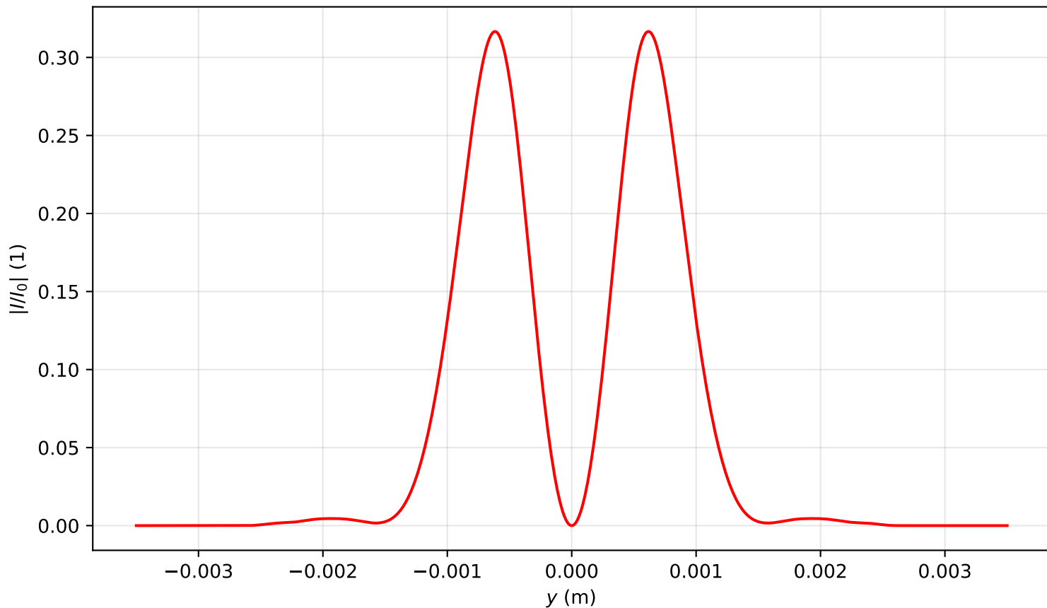
Intensity profile I(x=0, y, z=1.990)/I_0 , P_{in}=4.0P_{cr} , artificial time
